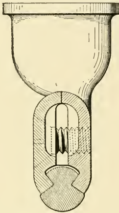
Fig. 187. Section Through Clamp Shown in Fig. 186
